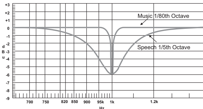
Notch Filter Q Diagram
