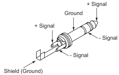
6.3 mm (1/4") Stereo Phone Plug
